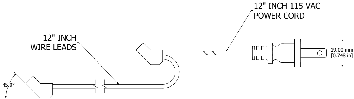
SIDE VIEW
